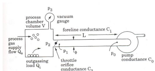
Figure 3.3 Geometry for gas throughput calculations.
